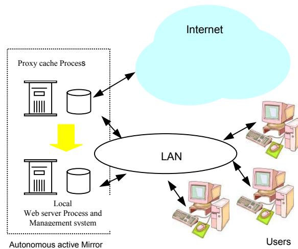
Figure 1: Network architecture
